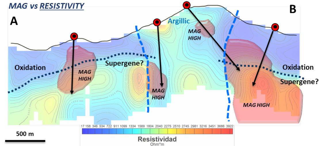
Resistivity Cross-section A-B
